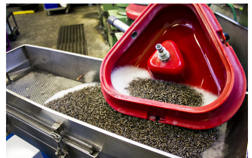
Tribofinition
